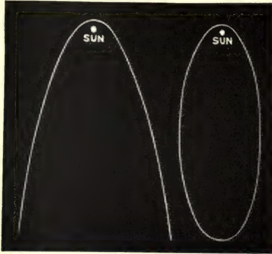
DIAGRAM OF A PARABOLIC AND AN ELLIPTIC ORBIT.
